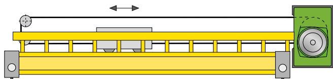
The AS 7 wire rope hoist used as horizontal towing equipment in systems manufacture.
